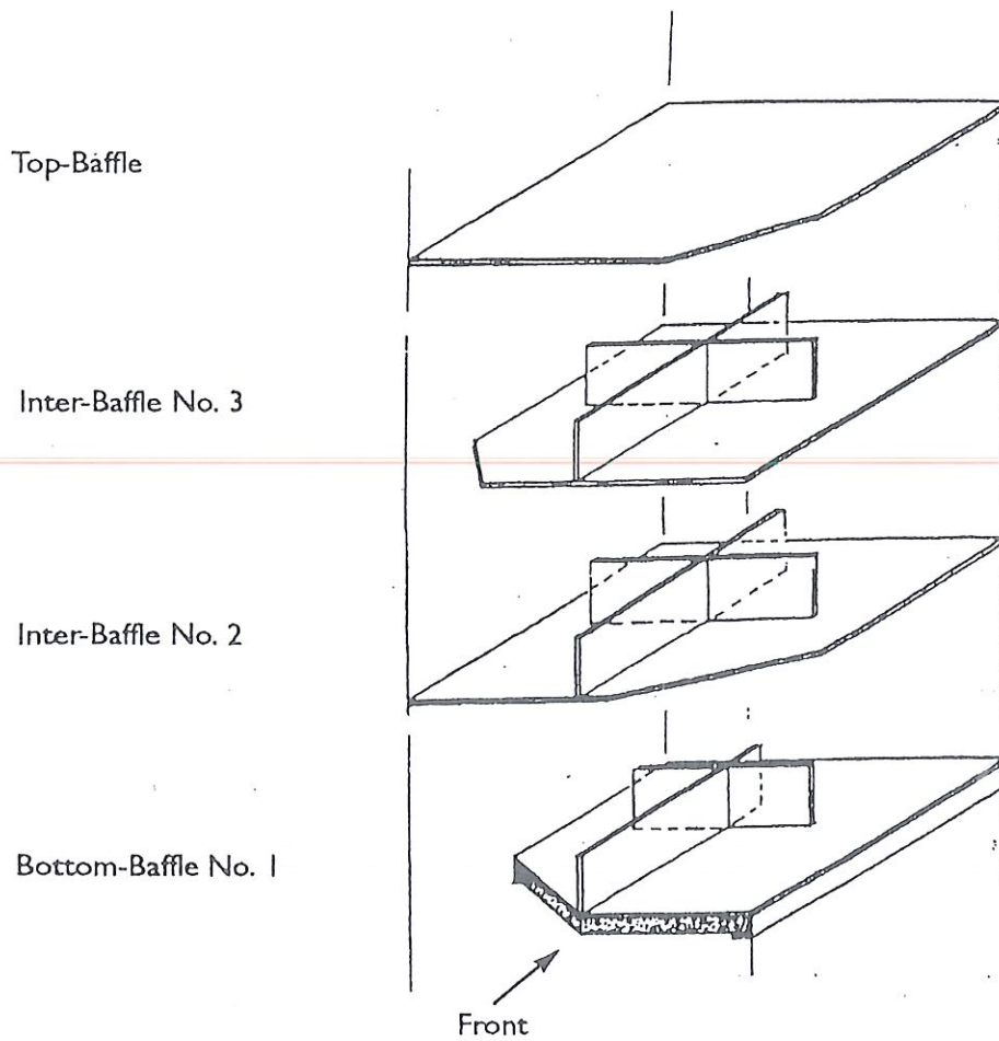
BAFFLE ASSEMBLY MERLIN BOILER 100.150 WATERWAY TOP
